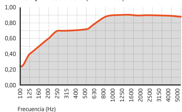
Absorption coefficient (Mineral Fiber)
